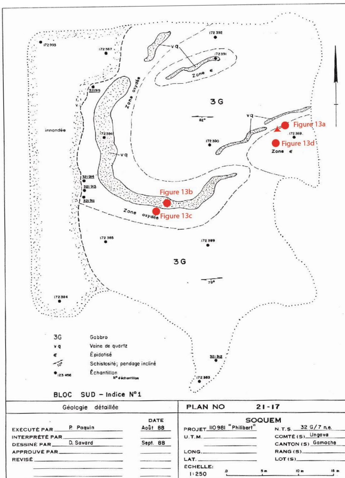
Figure 12: Geological map of the Philibert-I Showing, modified after GM 47926.
