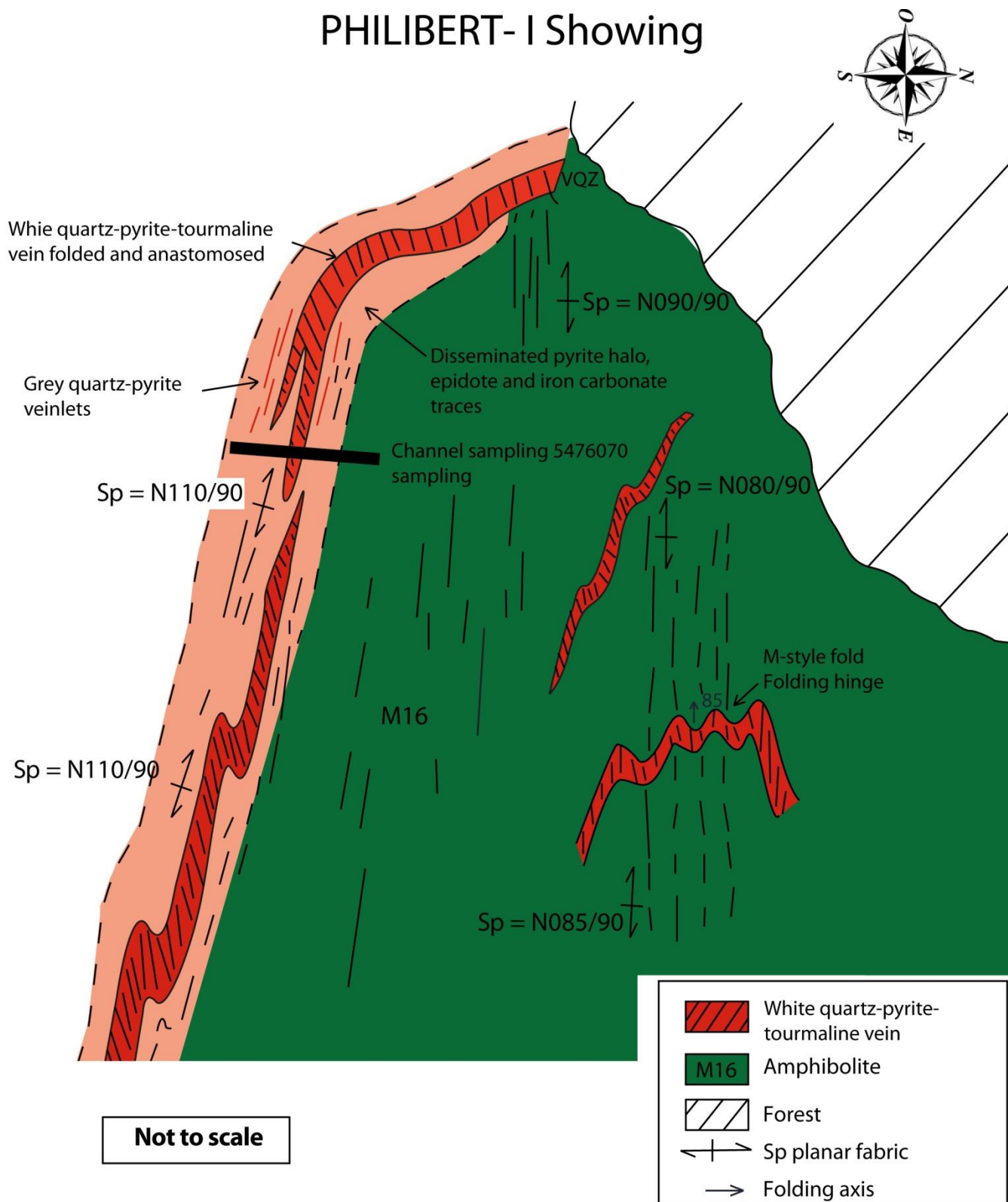
Figure 14: Plan view of the Outcrop – Sketch by Jérôme Augustin QP September 2018 (Laurentia(c))
