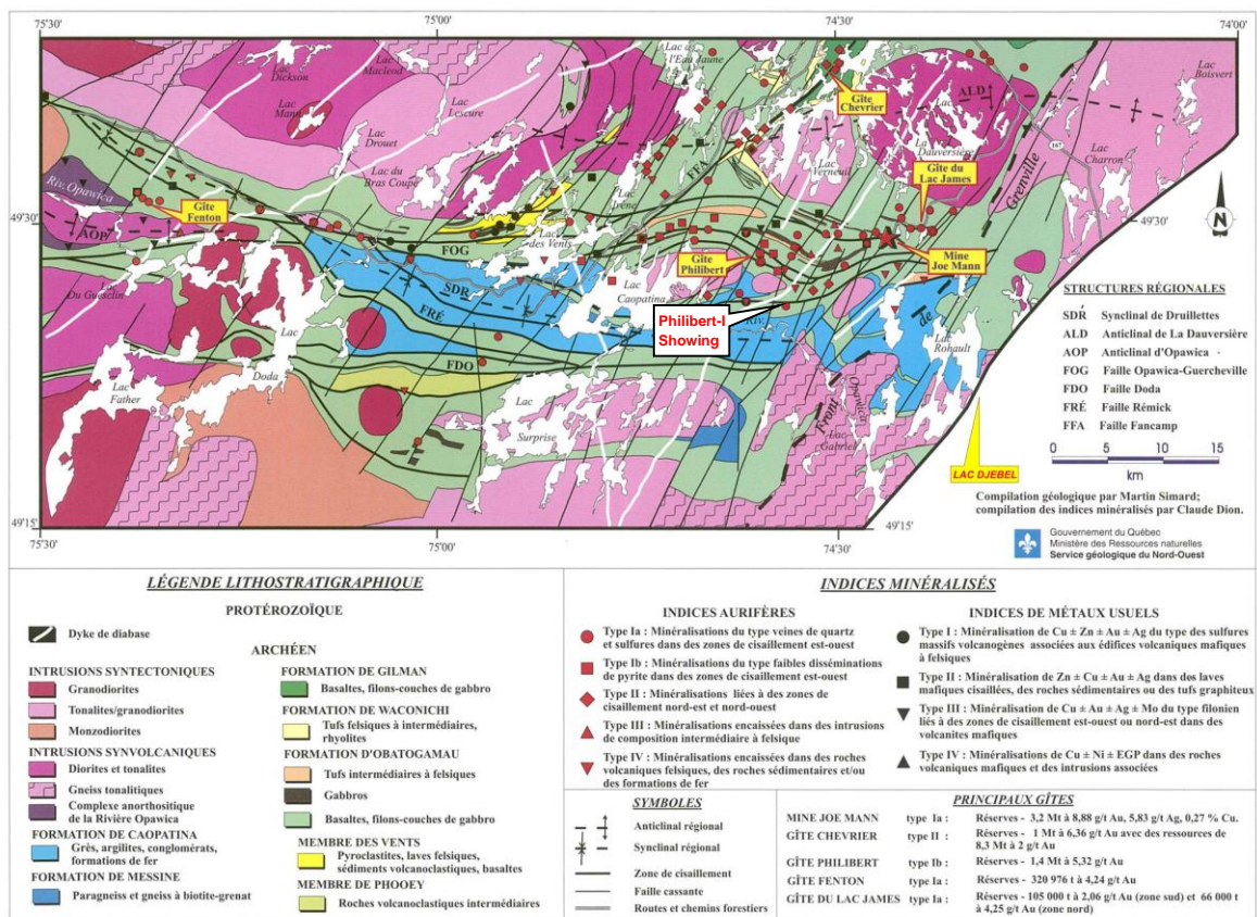
Figure 8: Regional geology of the Opawica Property (PRO 97-04).
